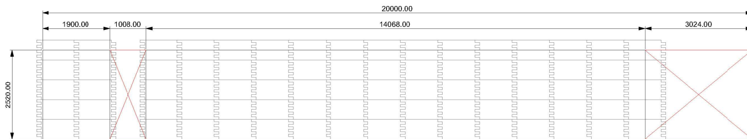
KIT "A" FOR H 2500 mm WALLS (80 tiles - up to 40 sqm)
